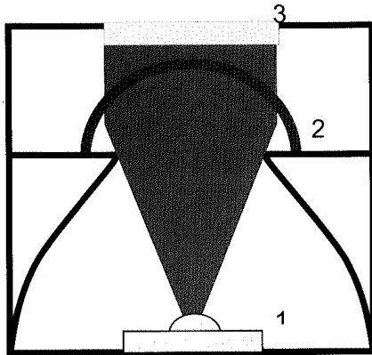
Fig. 5. Cross-section of the light cube: 1 = 4x LED (RGGGB); 2 = condenser lens; and 3 = interference filter.
