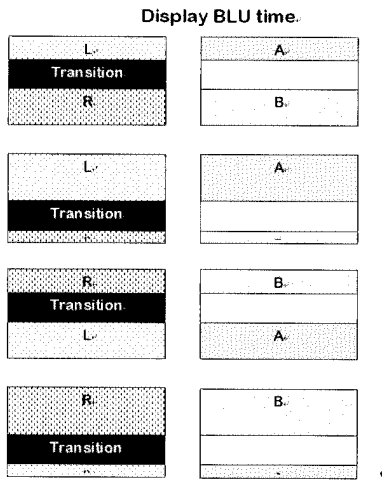
Fig. 2. Time synchronization between BLU and display driving.
